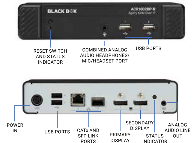
Agility Dual Monitor DisplayPort Receiver (ACR1002DP-R)
