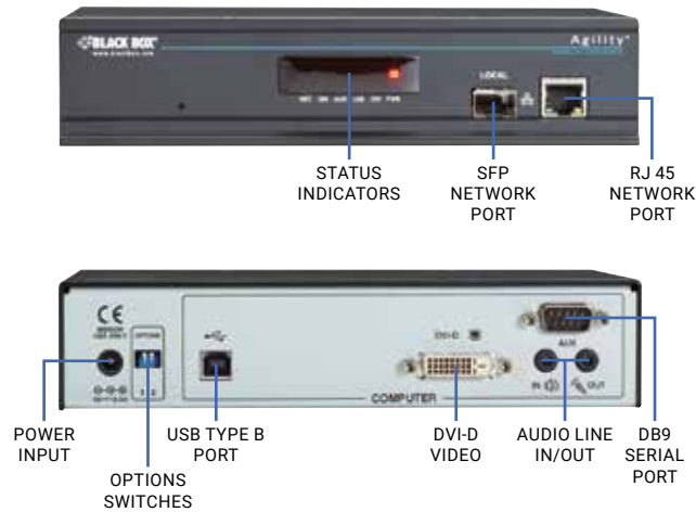
Agility Single Head DVI Transmitter (ACR1000A-T-R2)
