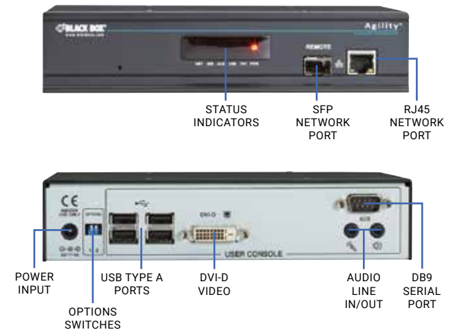
Agility Single Head DVI Receiver (ACR1000A-R-R2)
