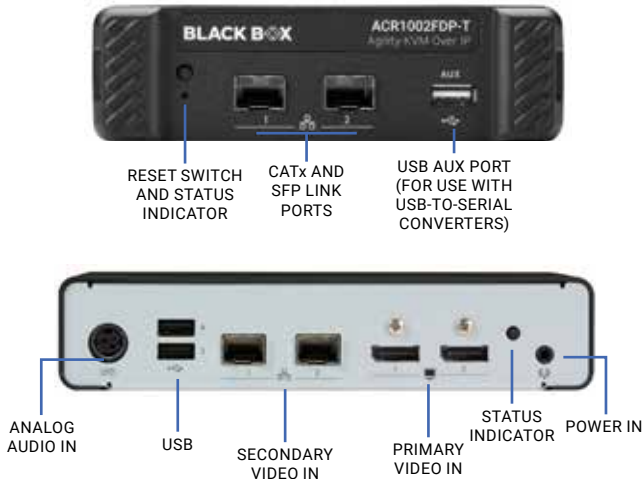
Agility Dual Monitor DisplayPort Transmitter (ACR1002DP-T)
