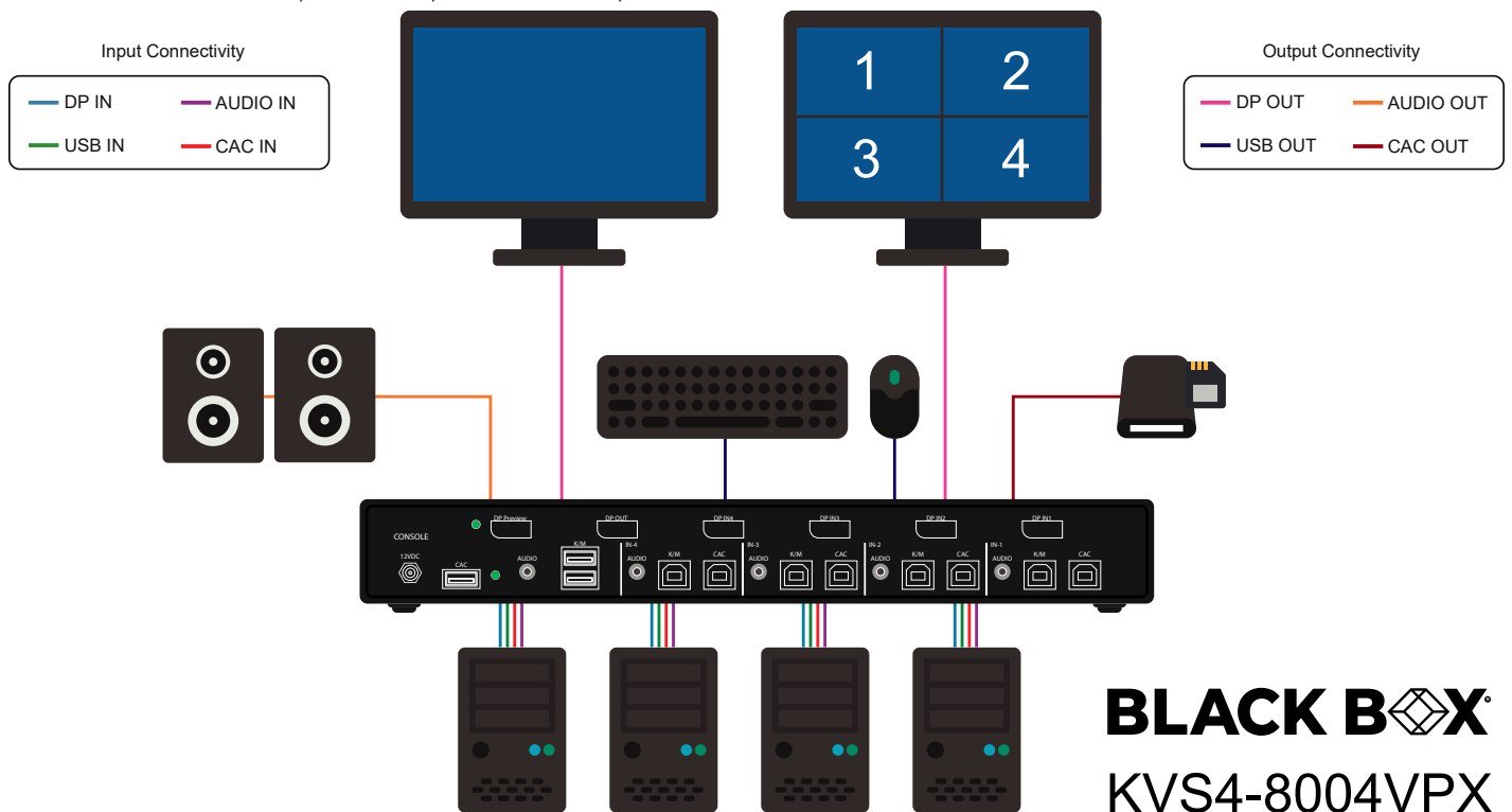
Figure 1-3: KVS4-8004VPX
