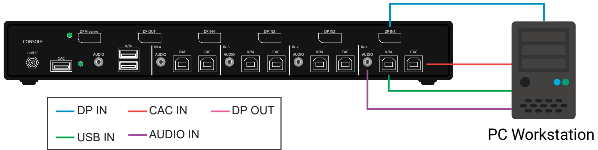
Figure 1-4: KVS4-8004VPX
